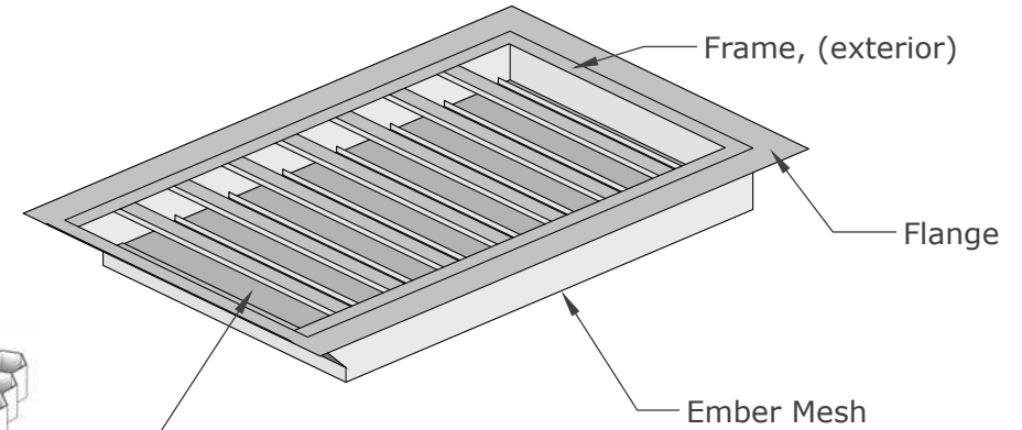
ISOMETRIC VIEW
