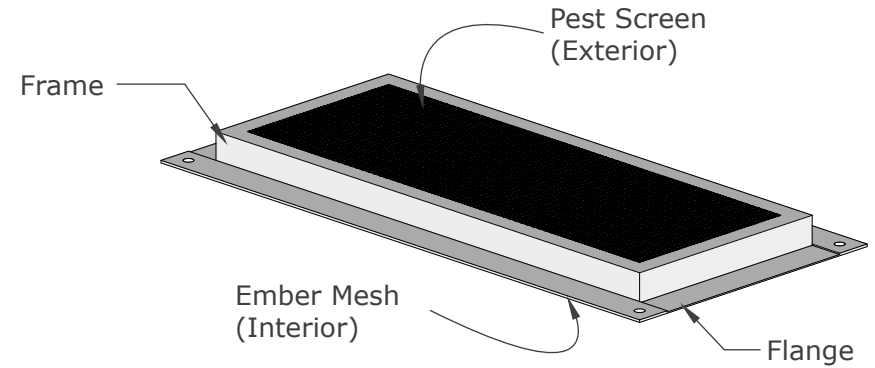
ISOMETRIC VIEW
