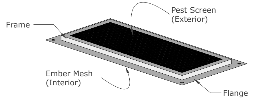
ISOMETRIC VIEW
