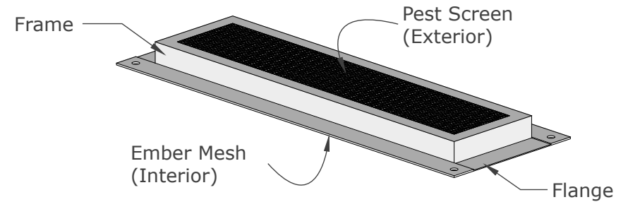
ISOMETRIC VIEW
