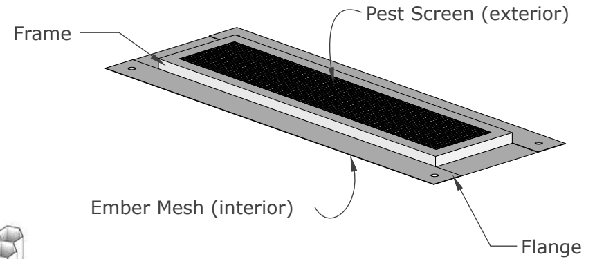
ISOMETRIC VIEW
