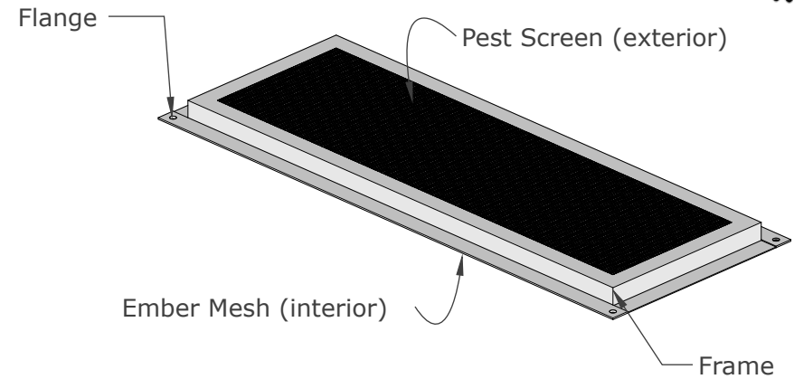
ISOMETRIC VIEW
