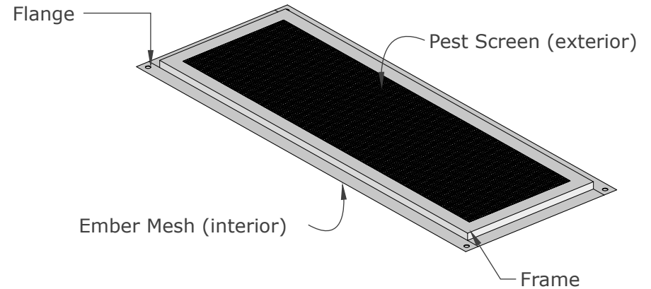
ISOMETRIC VIEW
