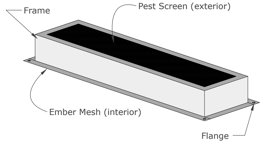
ISOMETRIC VIEW
